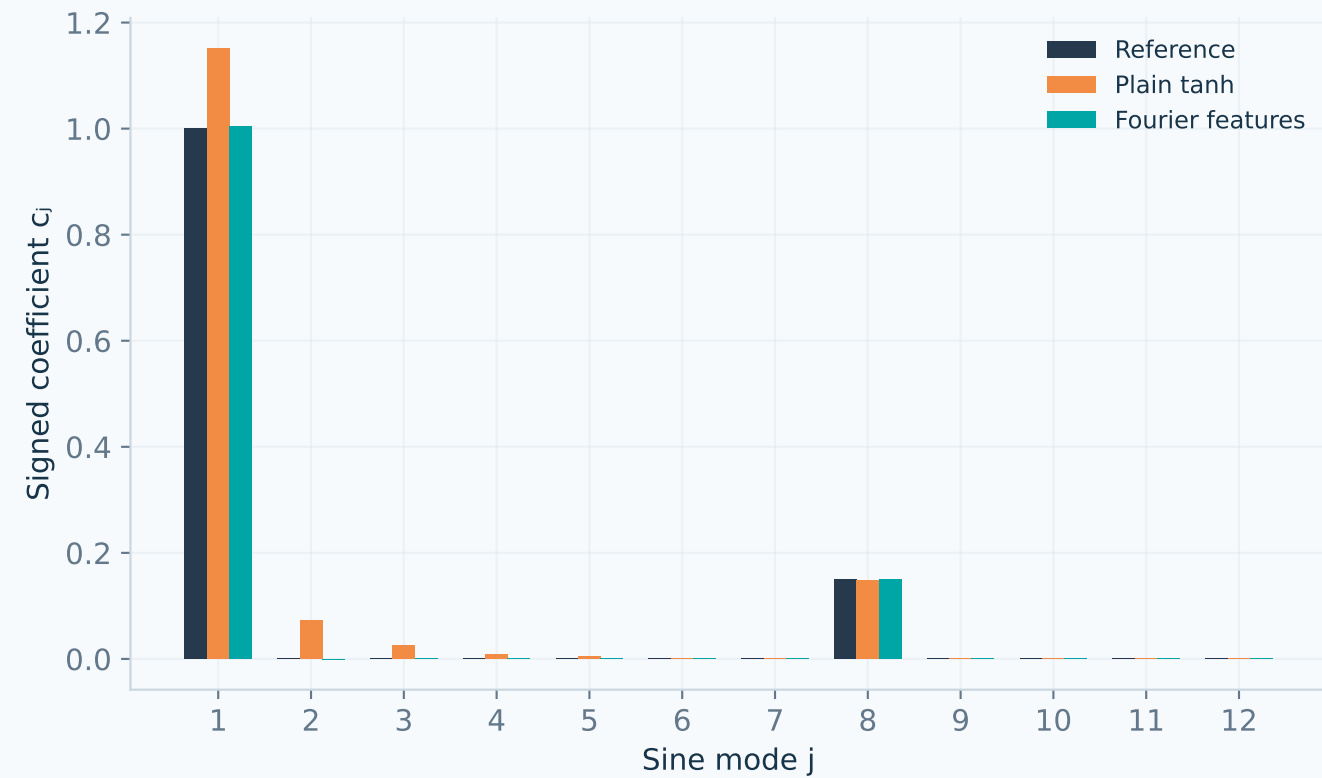
Which Fourier modes were recovered?
