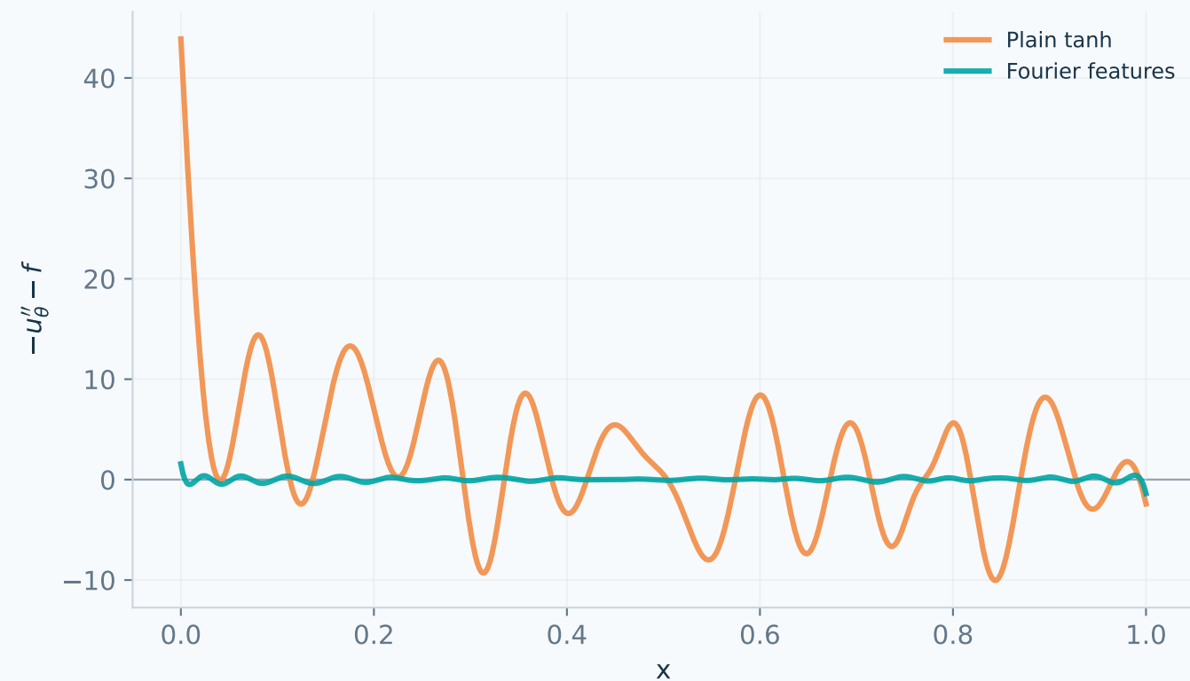
Which Fourier modes were recovered?
