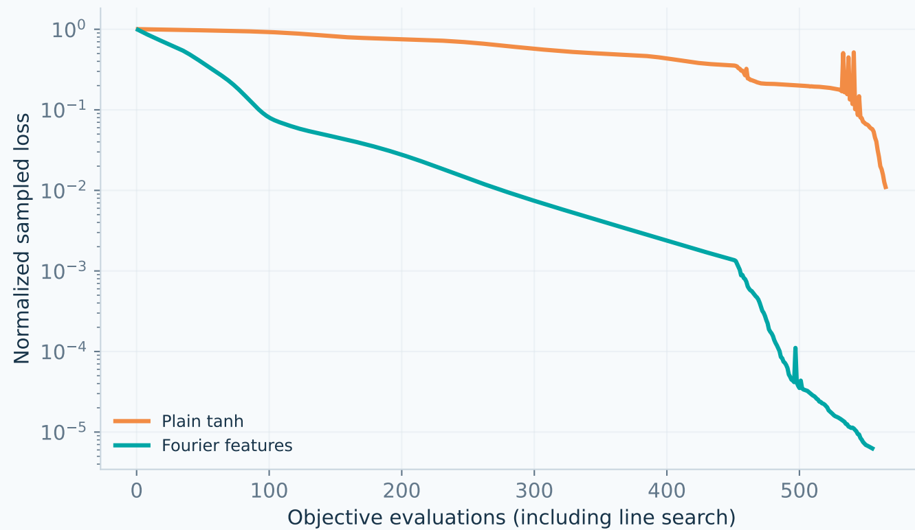
Same iteration limits; different evaluation counts
